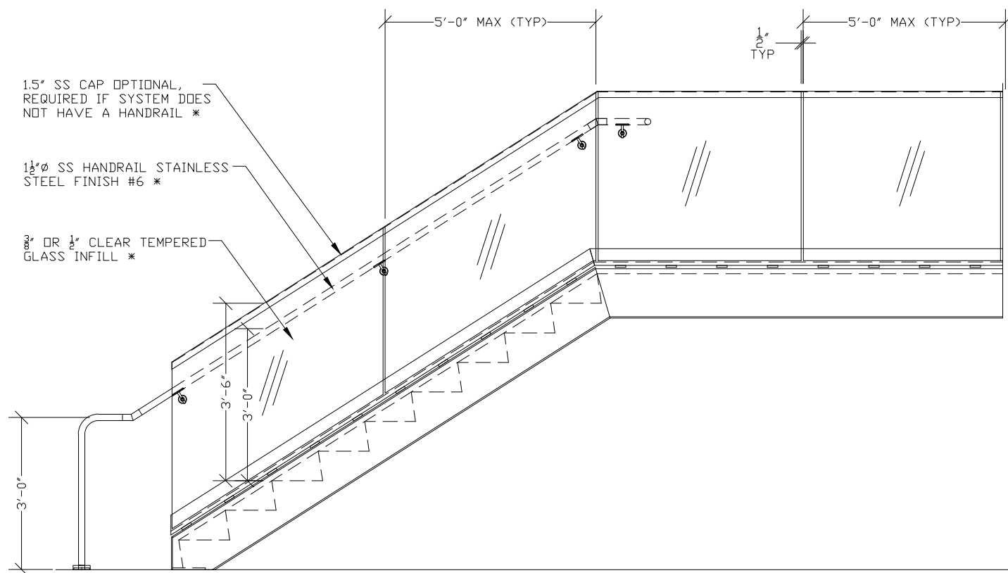
ELEVATION (SHOWING GLASS INFILL)
