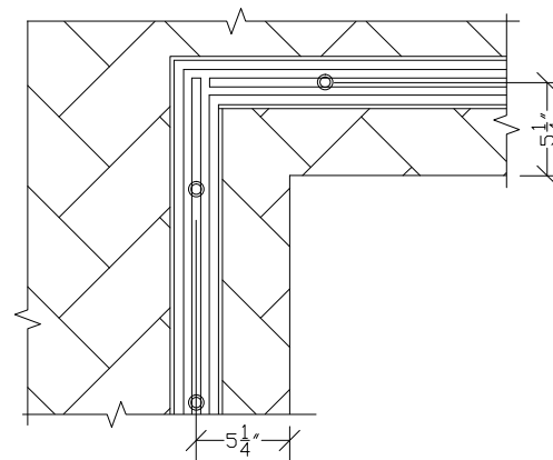
OUTSIDE CORNER TOP MOUNT
