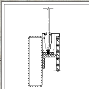
Fascia Mount
