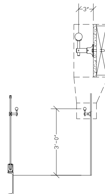
SECTION
