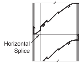
Horizontal Mullion (standard)
