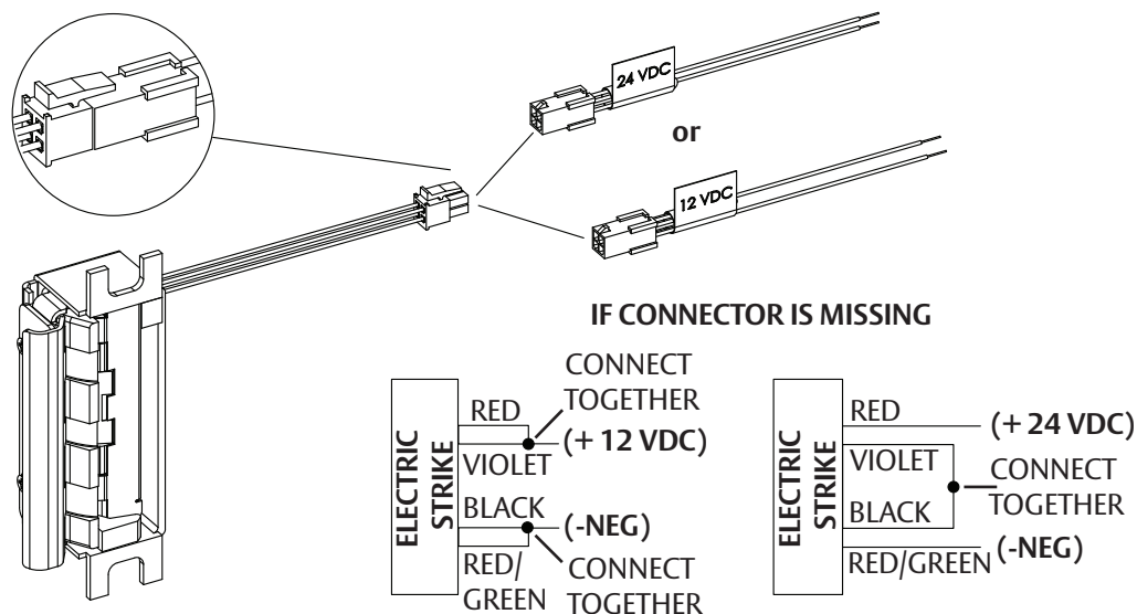
DIAGRAM 1: 12V to 24V CONVERSION
