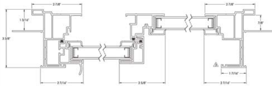
Brickmould 300 Single Slider HORIZONTAL ASSEMBLY
