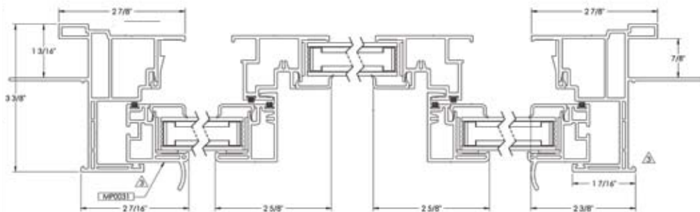
Brickmould 300 3-lite Slider HORIZONTAL ASSEMBLY
