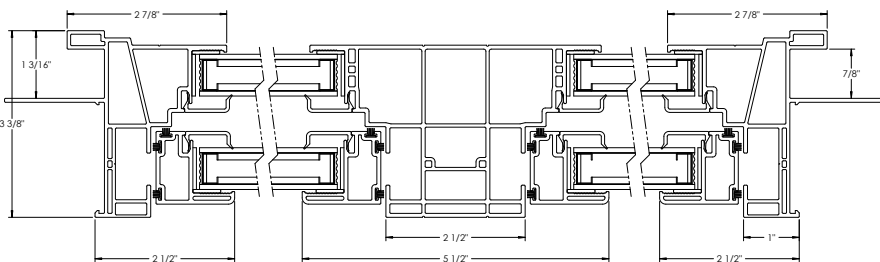
Brickmould 300 Single Hung Continuous Head & Sill HORIZONTAL ASSEMBLY
