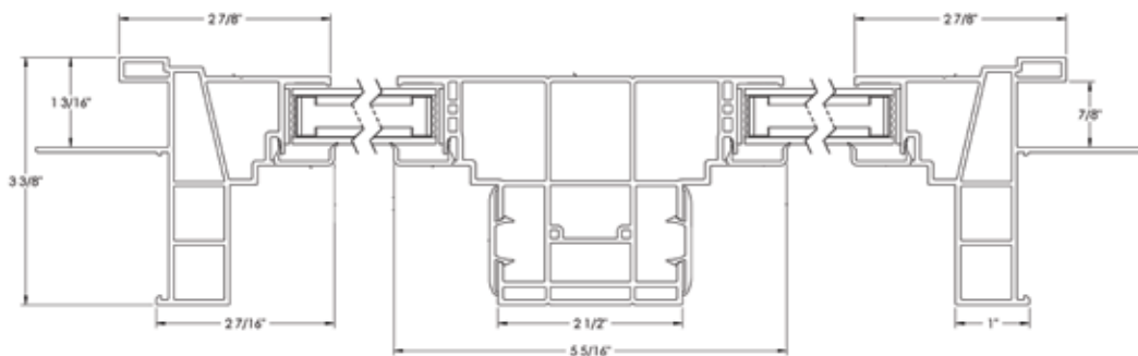
Brickmould 300 Picture Continuous Head & Sill Picture HORIZONTAL ASSEMBLY
