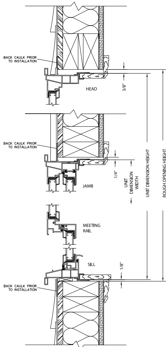
Brickmould 300 Single Hung Vinyl Siding Installation
