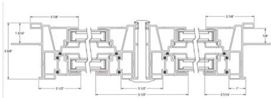
Brickmould 300 Single Hung Mullied HORIZONTAL ASSEMBLY
