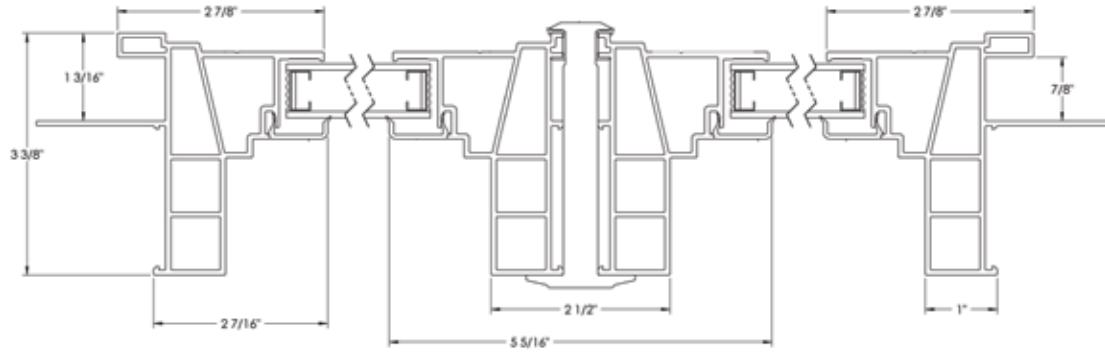
Brickmould 300 Picture Muller HORIZONTAL ASSEMBLY
