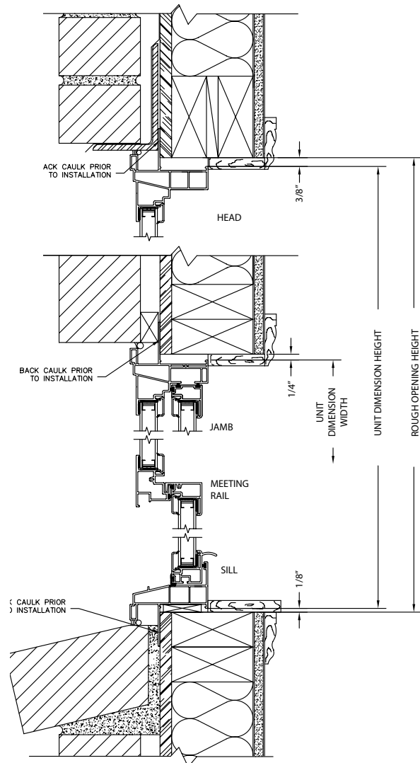
Brickmould 300 Single Hung 2 X 4 Brick Installation
