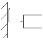
Reveal edge-buttcut wall condition
