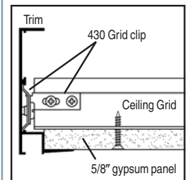
Drywall grid to trim (gypsum panel by others)
