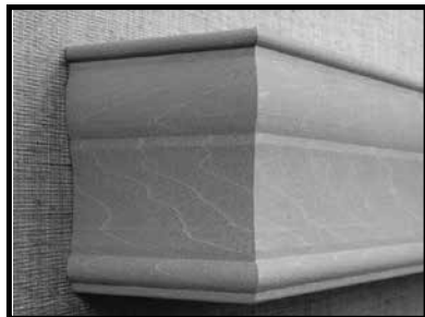
Majesty Valance 4 1/2" height 5/8" thick
