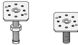
All TecCrete bases are available in Cornerlock Field Heads or Perimeter Heads shown above in standard and low profile versions.
