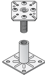
TecCrete Understructure, Low Profile 4" (102mm), and 5" (127mm) FFH
