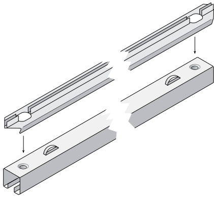
Steel Stringer with Gasket: 2' and 4'
