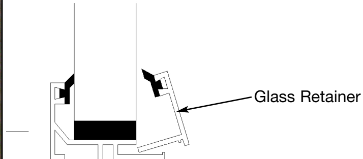
GLASS RETAINER INSTALLATION
