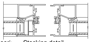
Rhino series Stacking detail (A)
