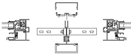
(B) Structural mullion detail
