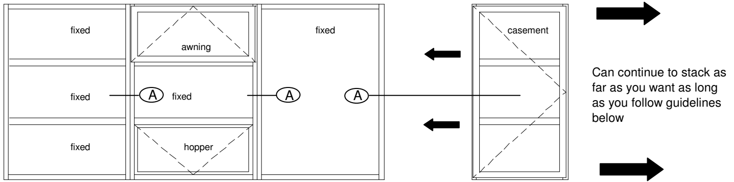
Rhino series Stacking detail (A)
