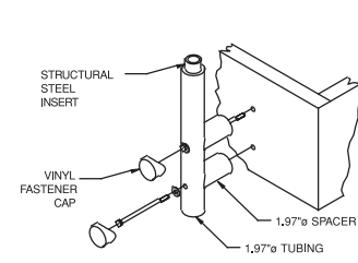
Fascia Mount
