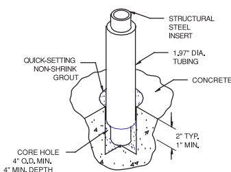
Core Mount
