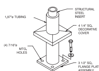
Flange Mount
