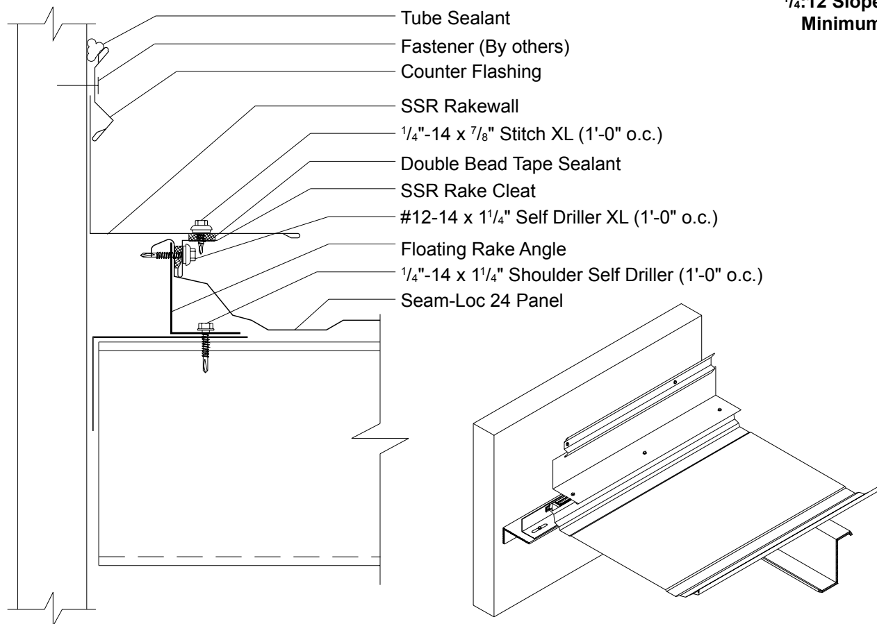
Rakewall with Reglet Option
