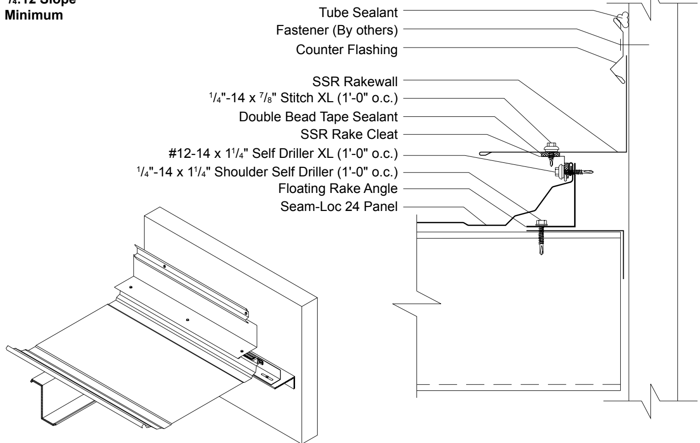
Rakewall with Reglet Option
