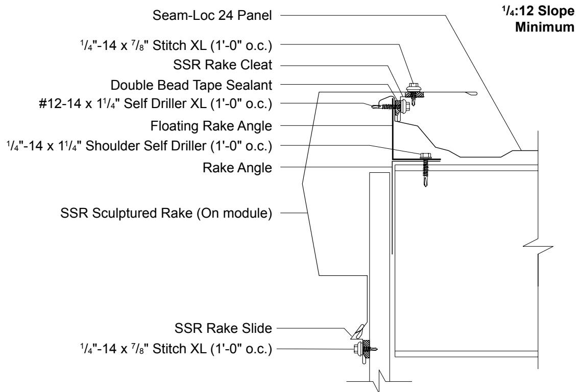
SSR Sculptured Rake (On Module)
