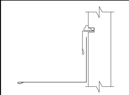
Rakewall with Reglet Option
