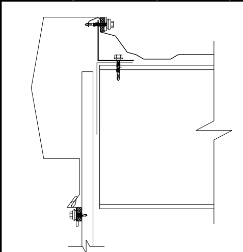
SSR Sculptured Rake (On Module)
