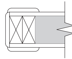
Wood Jamb (double 2 x 4 construction is needed for top and side jambs)
