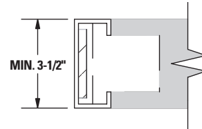
Hollow Metal Jamb (reinforced at hardware location)
