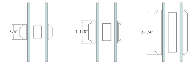
3/4" Vintage SDL
