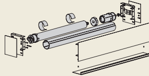
Easy-Set™ Fascia Hardware
