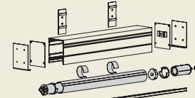
Easy-Set™ Cassette Hardware
