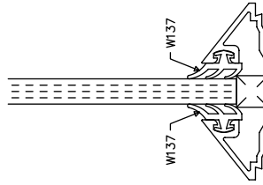
1/4" GLAZE
