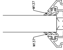
5/8" GLAZE
