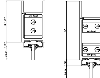
BOTTOM RAIL
