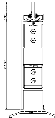
BOTTOM RAIL
