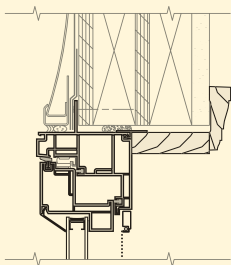
INTEGRAL NAILING FIN For wood framing and siding.
