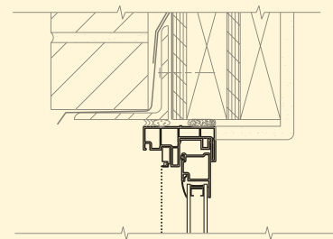
BLOCK FRAME For wood framing and brick veneer.
