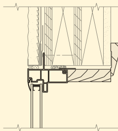
INTEGRAL NAILING FIN For wood framing and stucco.
