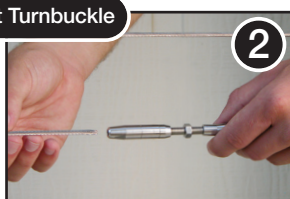
Surface Mount Turnbuckle
