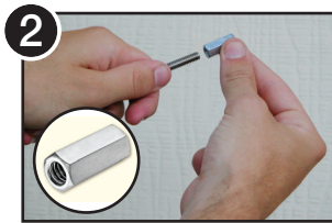
2 Spin Hanger Bolt Installation Tool onto the end of the bolt.
