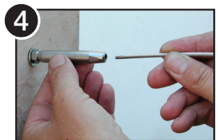
4 Insert cable all the way into Quick-Connect® fitting until it stops. Jaws will lock automatically.
