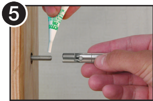
5 Apply a drop of high strength thread locking compound to threads.
