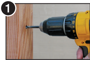
1 Drill 7/64" pilot hole (7/32" hole for 3/16" fitting). Harder woods may need larger hole.
