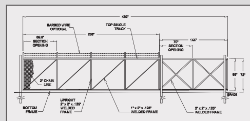
Chain Link Cantilever Gate (Detailed Example)
