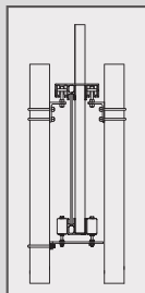
Track & Trolley Assembly (Double)
