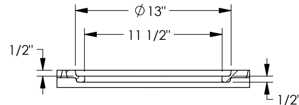
SECTION C-C SCALE 1 : 8
