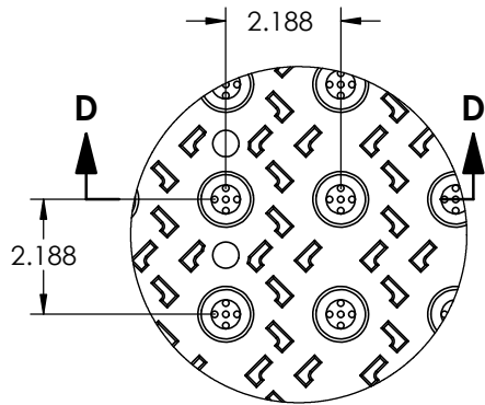
DETAIL E
