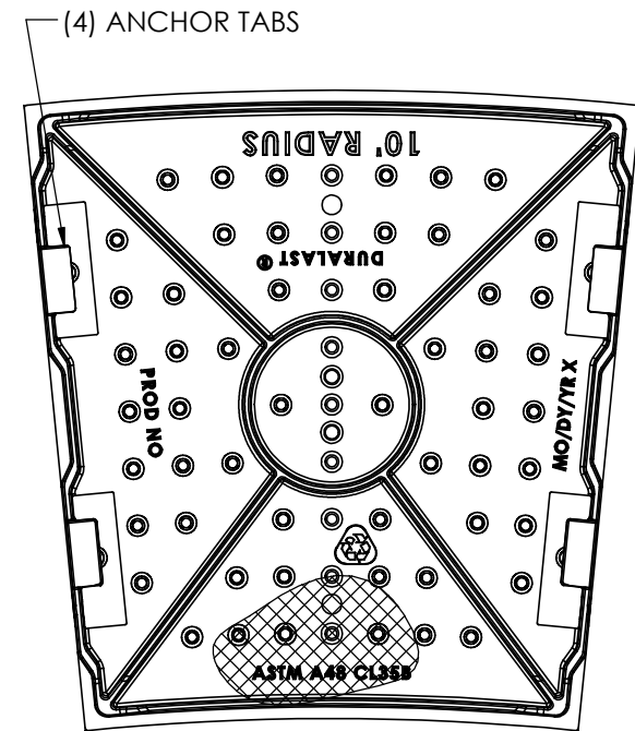
BOTTOM VIEW
