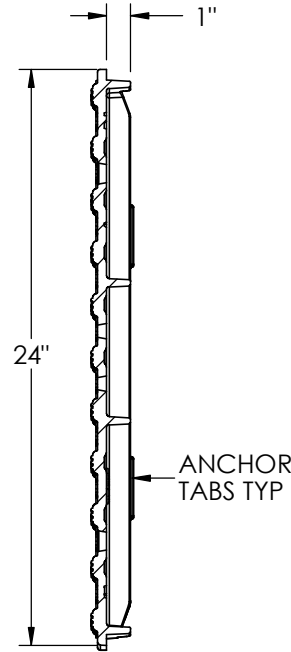
SECTION B-B
