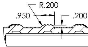
DETAIL C SCALE 1 : 4
