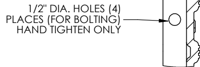
DETAIL C
