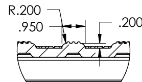
DETAIL C SCALE 1 : 4
