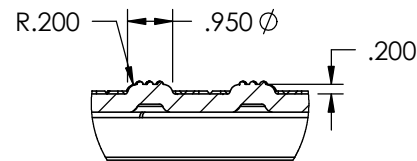
DETAIL C SCALE 1 : 4
