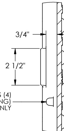
DETAIL C
