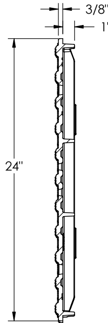
SECTION B-B
