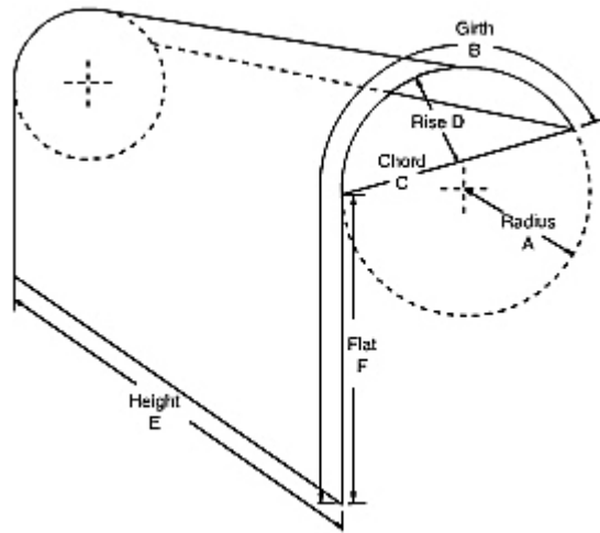
BENT GLASS DIMENSIONS
