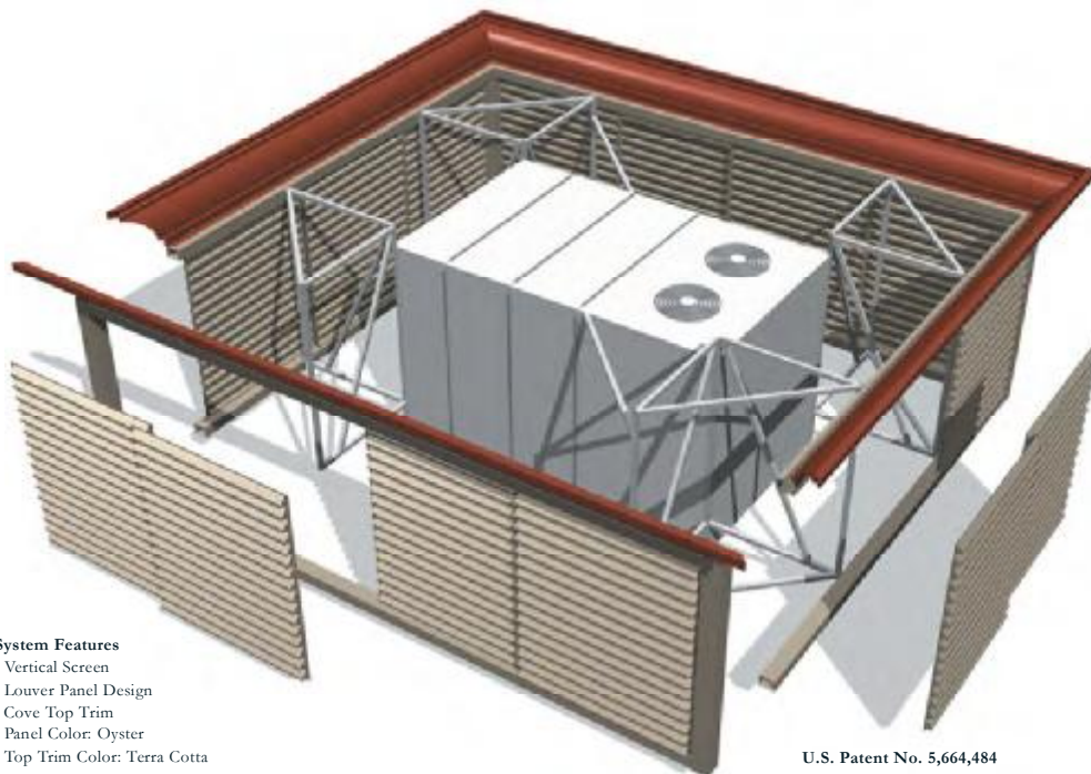
52" Louver Panels
