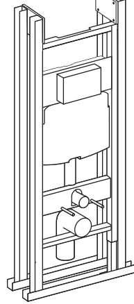
Metal frame in-wall installation, front activation.
