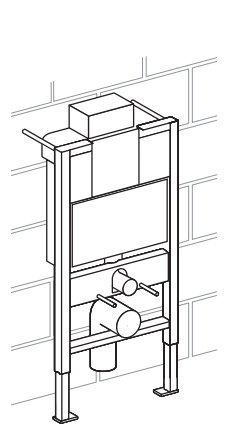
Pre-wall installation, top or front activation.
