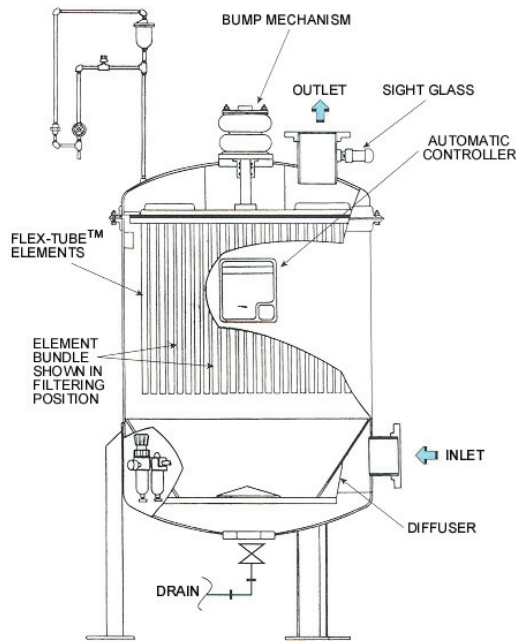
Ref. 3 Regenerative D.E. Filter
