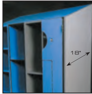
Single End Panel with 20° Sloped Top
