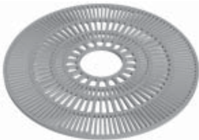
R-8855-1 • 72" Round 16" diameter expandable tree opening. Bolted light opening grates (9" x 17.143" x 4.5") for use with sub-grade lighting. 495 pounds per set. Supplied with light grates, none shown.
