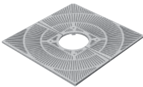
R-8714-A • 60" x 60" 18" diameter tree opening. .375" slot openings. Four 1" diameter holes for staking tree. 520 pounds per set. Available with light openings.
