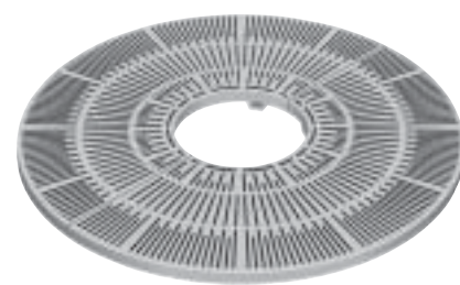
R-8870 • 60" Round 18" diameter expandable tree opening. .25" slot openings. 375 pounds per set. Available with light openings. R-8870 is also a Los Angeles approved grate.
