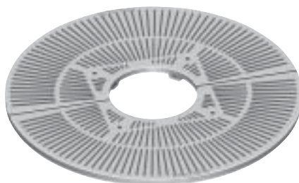
R-8869-A • 60" Round 18" diameter tree opening. .375" slot openings. Four 1" diameter holes for staking tree. 356 pounds per set. R-8869-ALA Order as R-8869-ALA for Los Angeles approved grate.
