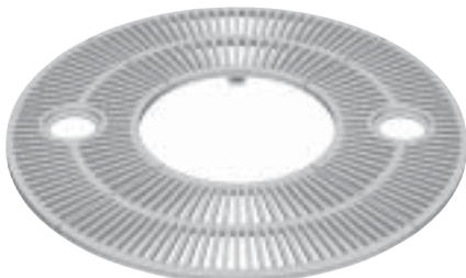
R-8860 • 93" Round Four-piece, with 40" diameter opening. For use with sub-grade lighting. 9.5" openings. Support at section joint is required — furnished by installer. 640 pounds per set. Also available without light openings.
