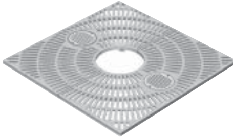
R-8742-A1 • 60" x 60" 18" diameter expandable tree opening. Bolted light opening grates (10.375") for use with sub-grade lighting. 396 pounds per set. (Available without light openings, order as R-8742-A . 418 pounds per set.)
