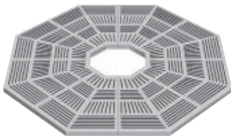
R-8953 • 64" Octagon 16" octagonal expandable tree opening. 516 pounds per set. No tree guards available for octagonal openings.
