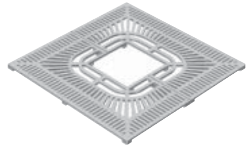
R-8768 • 48" x 48" 16" square tree opening. 190 pounds per set.
