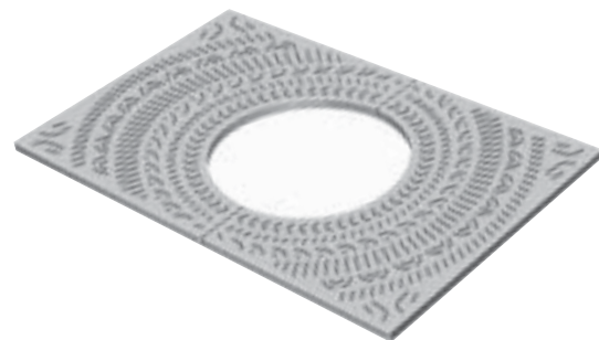
R-8819 • 48" x 72" 30" diameter tree opening. .375" typical slot openings. 390 pounds per set.
