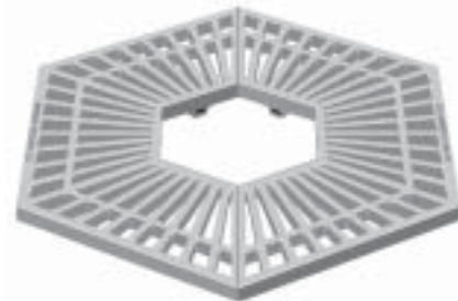
R-8950 • 44.5" Hex 16.5" hexagon tree opening. 345 pounds per set.
