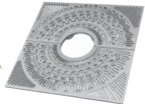
R-8757 • 48" x 48" 14" diameter tree opening. .375" typical slot openings. 306 pounds per set. Available with light openings. Order as R-8757-LA for Los Angeles approved grate.
