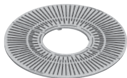
R-8830-A1 • 48" Round 18" diameter expandable tree opening. .25" slot openings. 252 pounds per set. (Available with light openings, order as R-8830-1 . 268 pounds per set.) R-8830-A1 or R-8830-1 are also Los Angeles approved grates.
