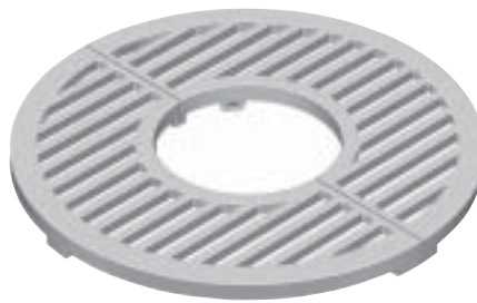
R-8825 • 30" Round 12" diameter tree opening. 80 pounds per set.
