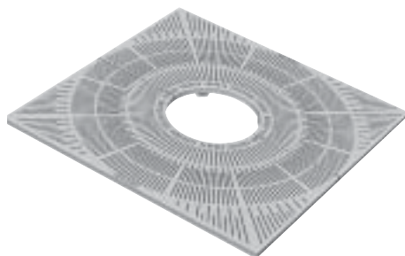
R-8709-A • 72" x 72" 24" diameter expandable tree opening. .25" slot openings. 750 pounds per set. Available with light openings.
