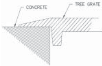
RETROFIT DETAIL
