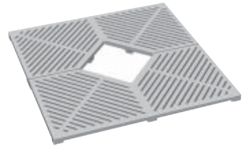
R-8724-A • 48" x 48" 15" square tree opening. .375" slot openings. 320 pounds per set. R-8724-A is also a Los Angeles approved grate.
