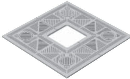
R-8737-B • 72" x 72" 23" square tree opening. Bolted light opening grates (10.375") for use with sub-grade lighting. .25" slot openings. 645 pounds per set. (Available as 60" x 60" square, order as R-8737-C . Also available with 30" square opening. 400 pounds per set.)
