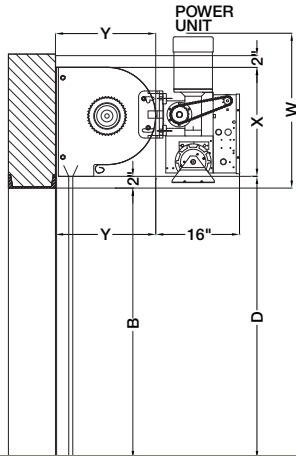
SECTION (FACE MOUNT)
