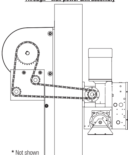
Through - wall power unit assembly
