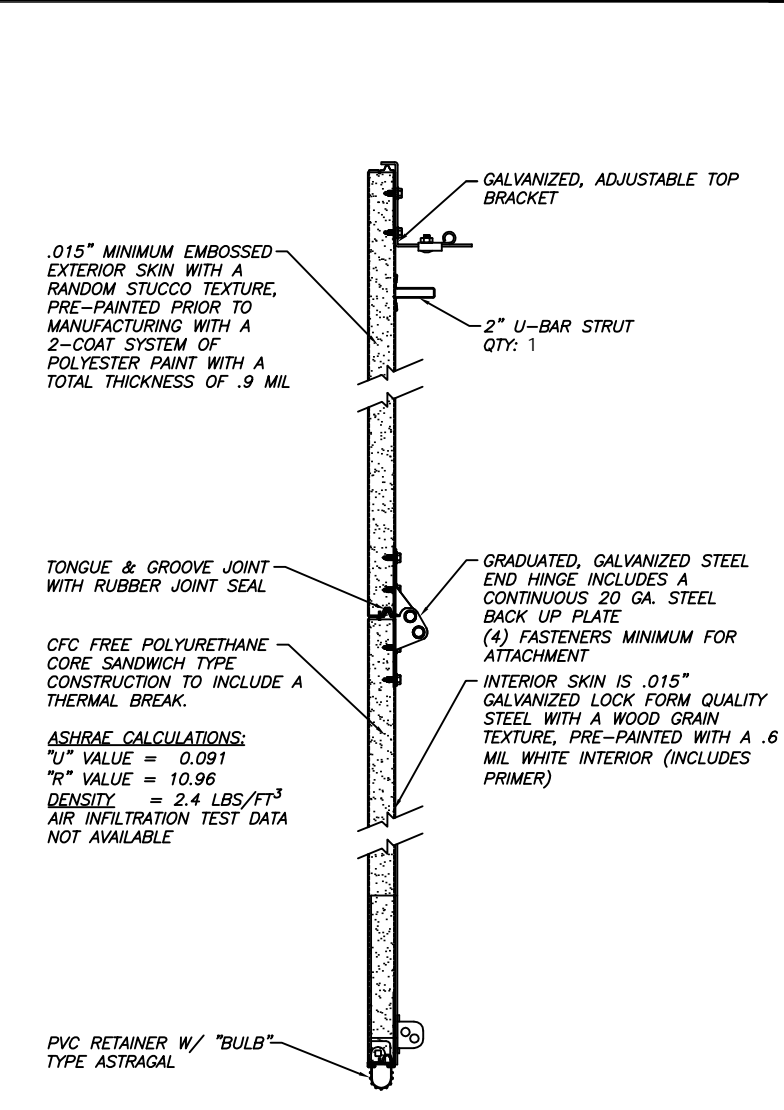
4 SECTION CONSTRUCTION
