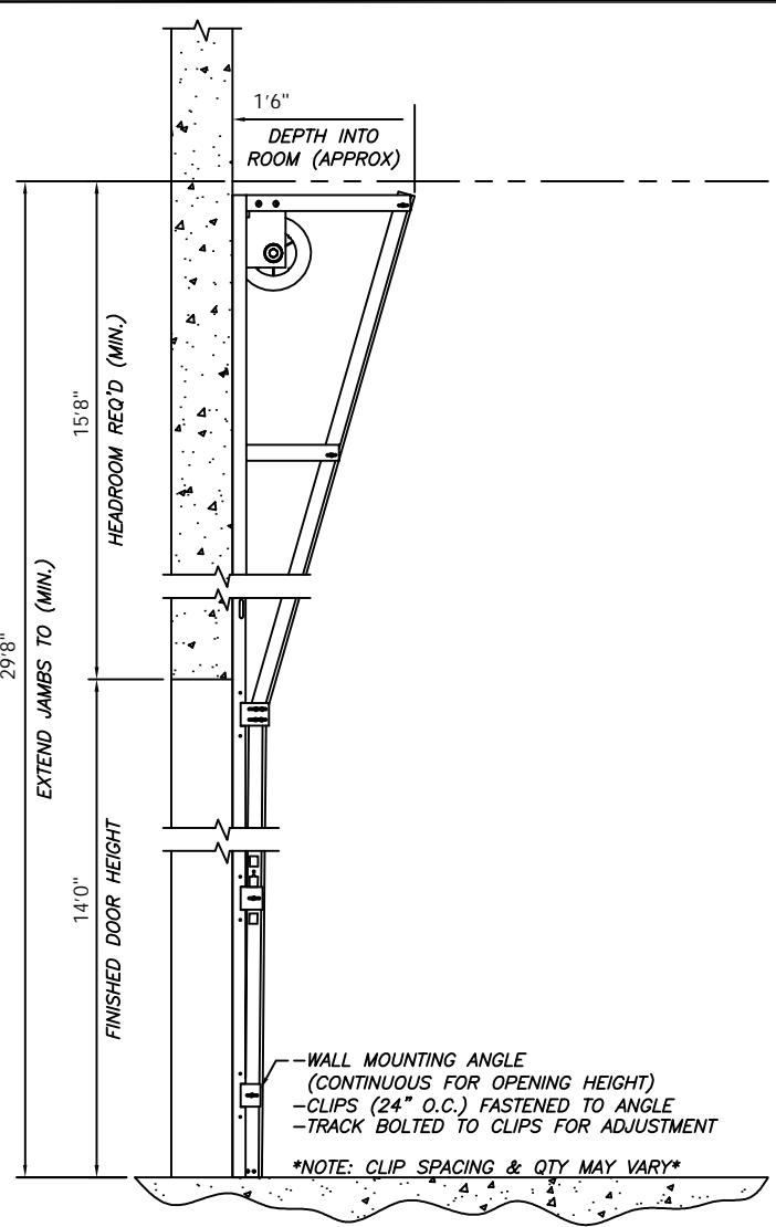
3 VERTICAL - BREAKAWAY
