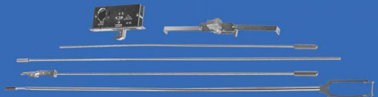
MS Series 5-Point Locking Hardware
