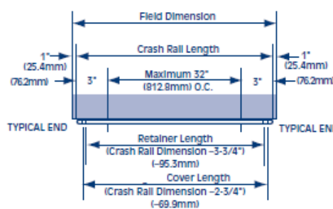
Typical Straight Length
