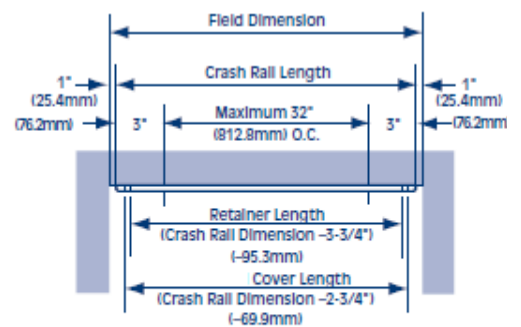
Typical Straight Length with Typical Ends
