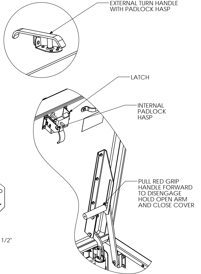
HARDWARE DETAILS
