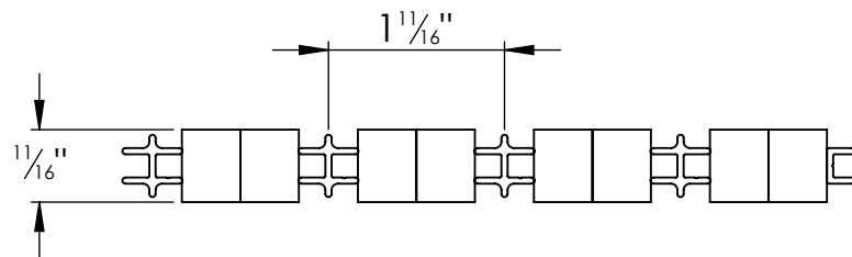
WIDTH VIEW
