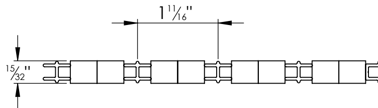
WIDTH VIEW
