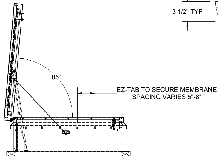
DETAIL D
