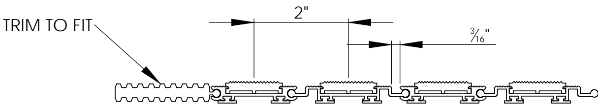
WIDTH VIEW
