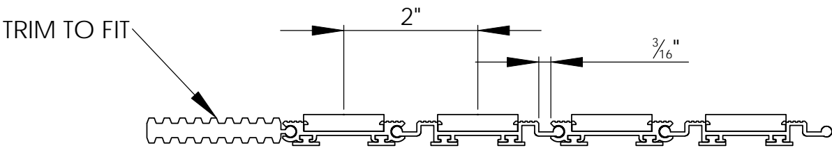
WIDTH VIEW
