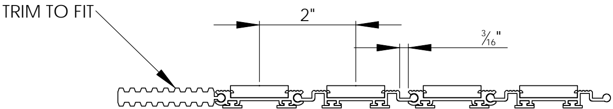
WIDTH VIEW
