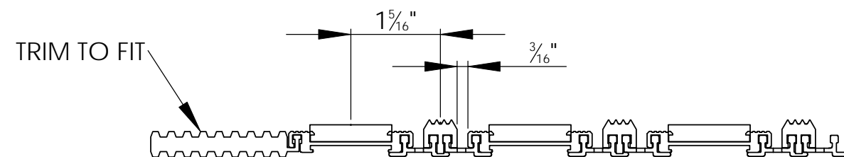
WIDTH VIEW
