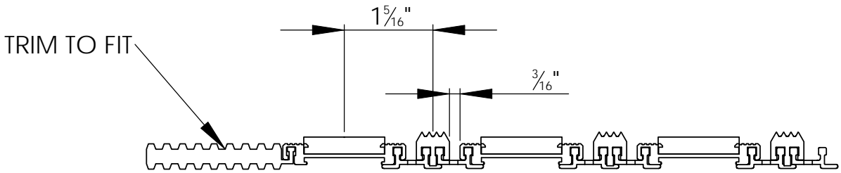
WIDTH VIEW
