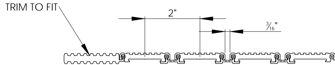
WIDTH VIEW
