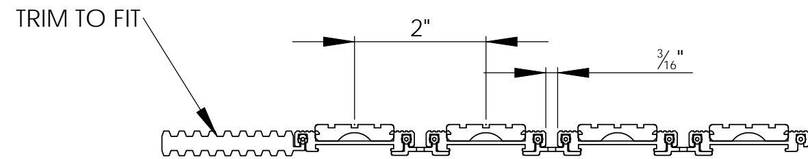
WIDTH VIEW
