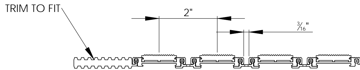
WIDTH VIEW
