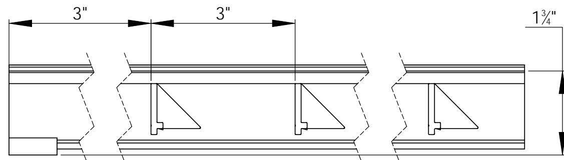
LENGTH VIEW
