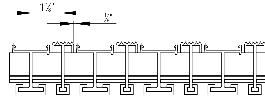
WIDTH VIEW
