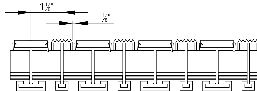
WIDTH VIEW
