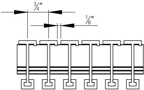
WIDTH VIEW
