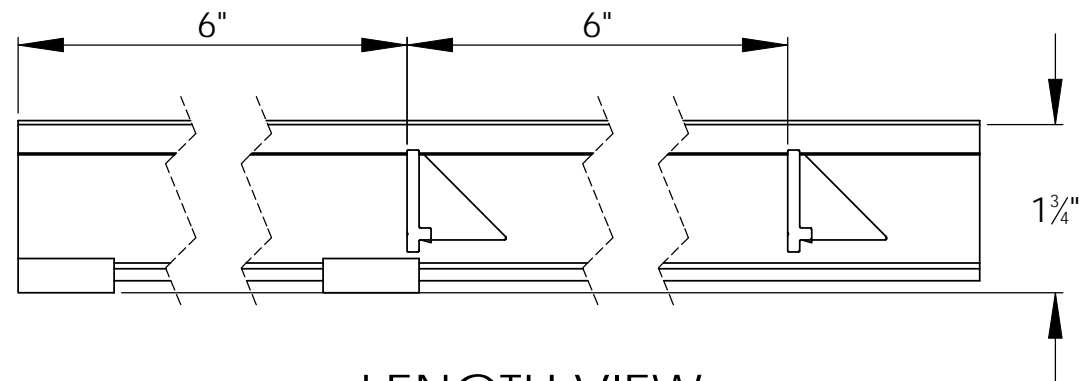
LENGTH VIEW
