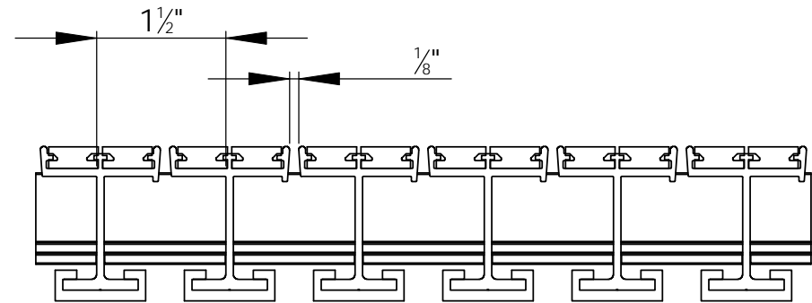
WIDTH VIEW
