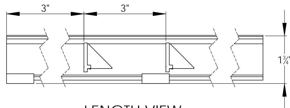
LENGTH VIEW
