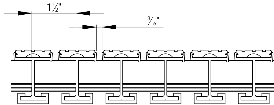
WIDTH VIEW
